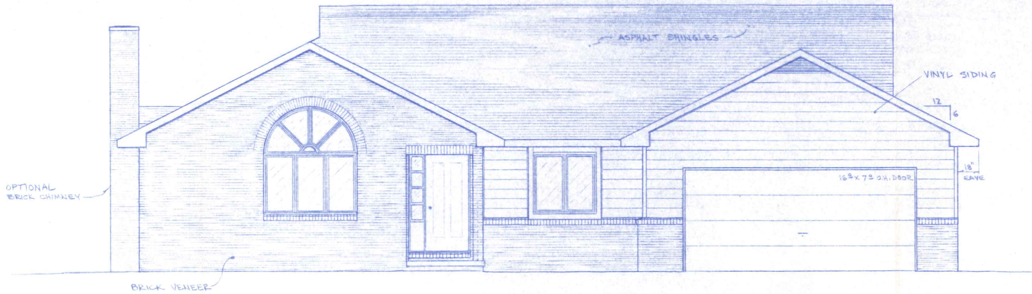
FRONT ELEVATION 1/4" = 1'-0"
