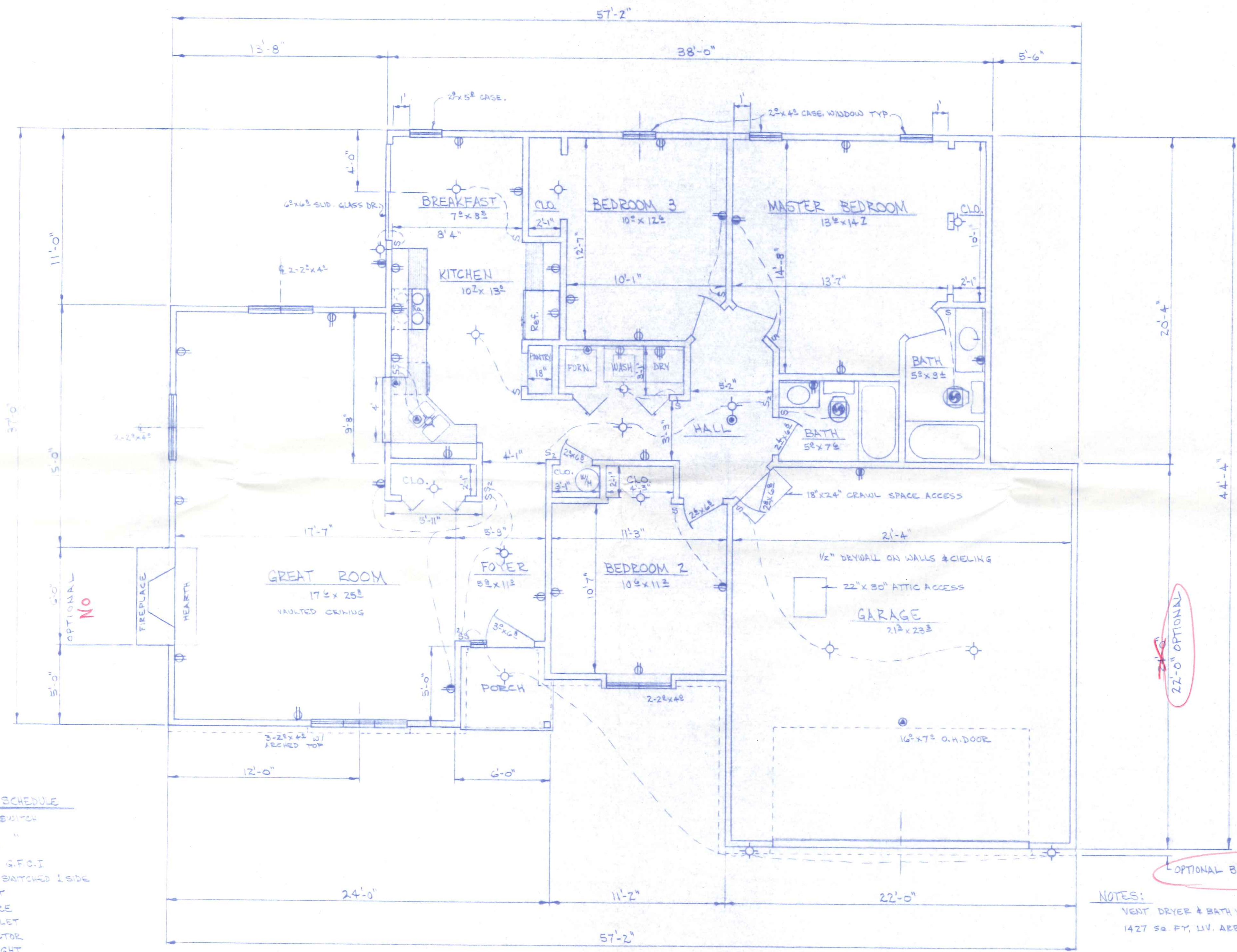
FLOOR PLAN 1/4" = 1'-0"
