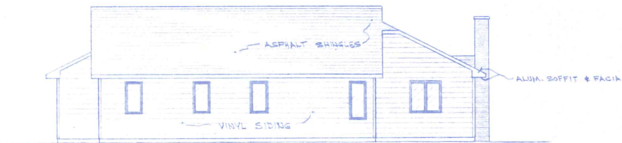
REAR ELEVATION 1/8" = 1'-0"
